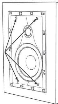
Figure 5: Tightening the Roto-Lock Screws
