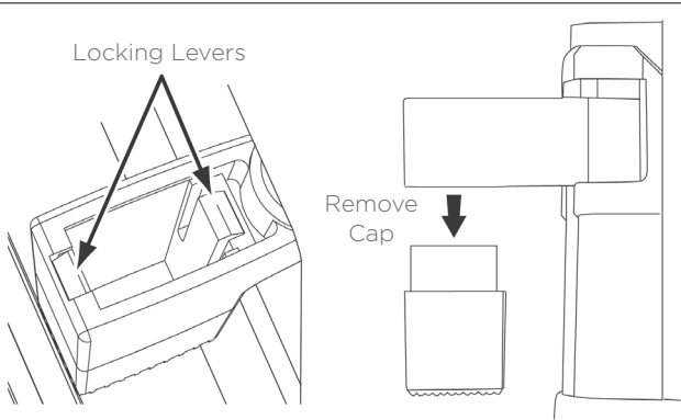
Figure 4: Removing the Caps from the Roto-Lock Toggle Feet
