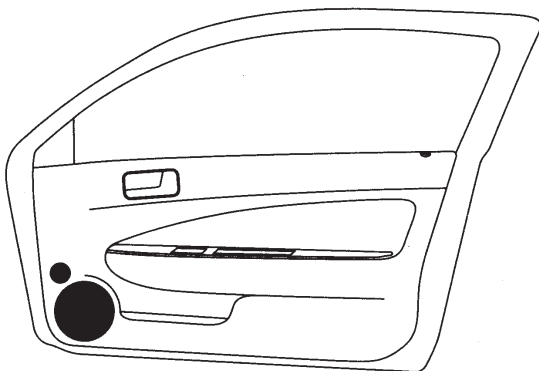
DIAGRAM H: COMPONENT CONFIGURATION - More Desirable Door Speaker Placement
