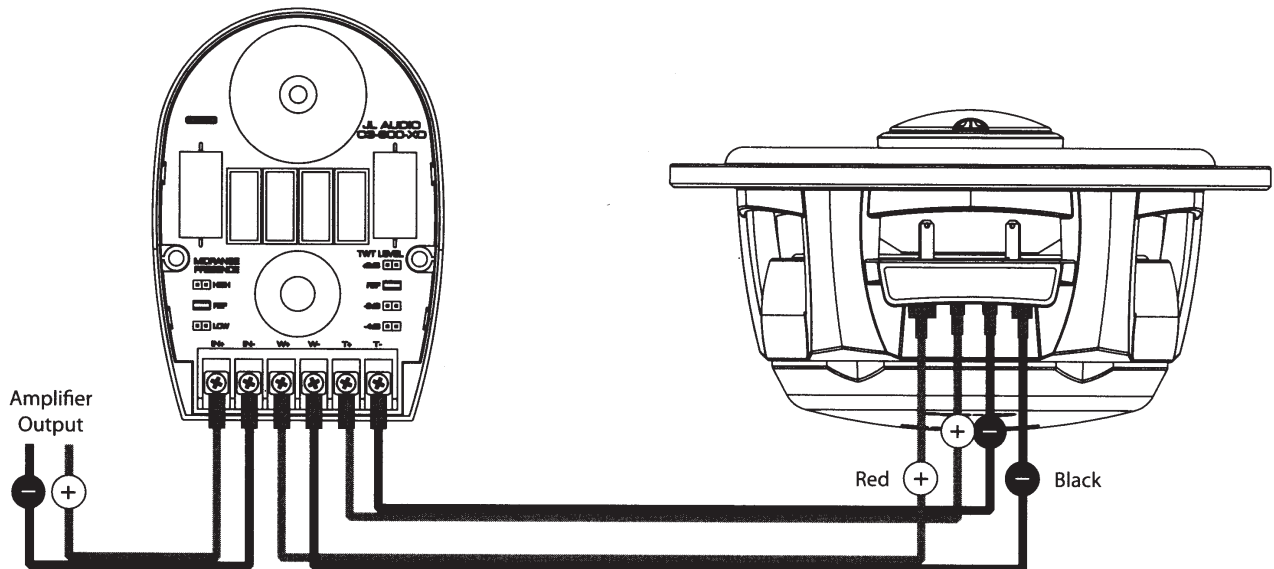
DIAGRAM B: Coaxial System Wiring
