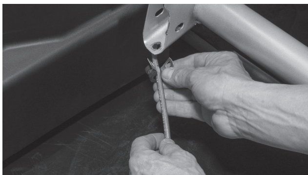
Step 7 - Wrap the brake line with the strip of adhesive backed foam tape included in the box. Note: This step is to prevent the brake line from rattling against the enclosure under high bass output and any chaffing due to movement of the brake line while the vehicle is in motion.
