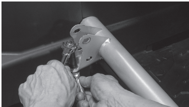
Step 6 - Remove the cable clamp from the brake line.
