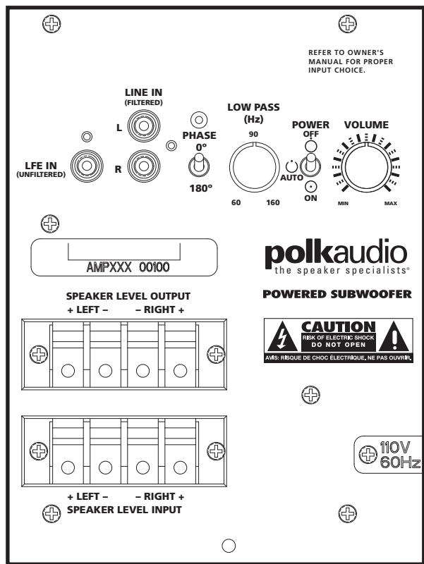
Figure 10 - PSW303 Controls
