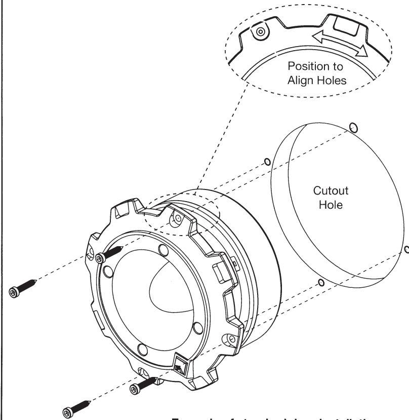
Example of standard door installation
