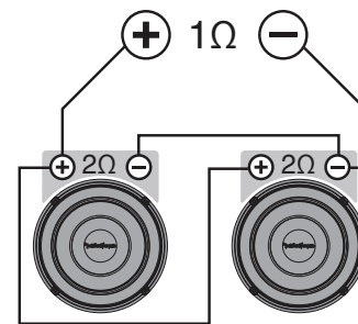
(2) 2 ohm SVC Speaker = 1 ohm Load
