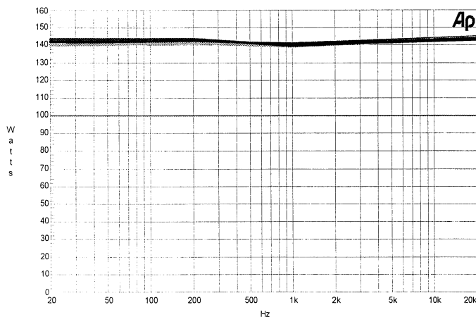
actual power measured into 2 Ohm loads
