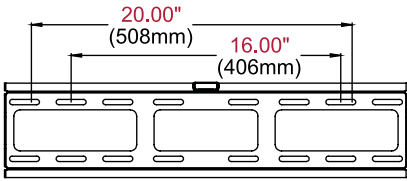
WALL PLATE DETAIL
