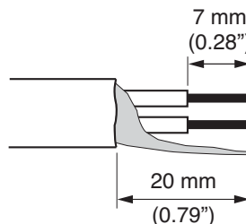
Shielded cable
